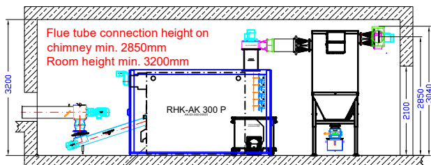
Multicyclone with ash bin 40 Liter Ash bin 400 Liter direct
