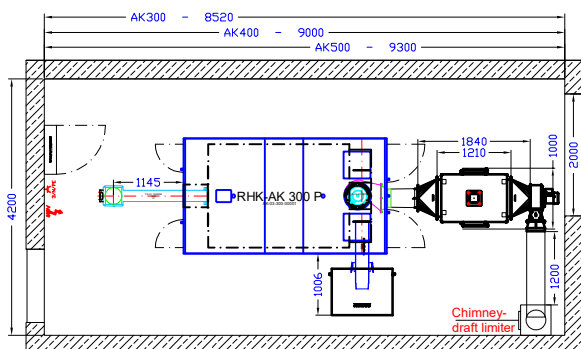
Multicyclone with de-ashing 900 Liter
