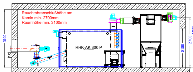
Multicyclone with ash bin 240 Liter Ash bin 400 Liter direct
