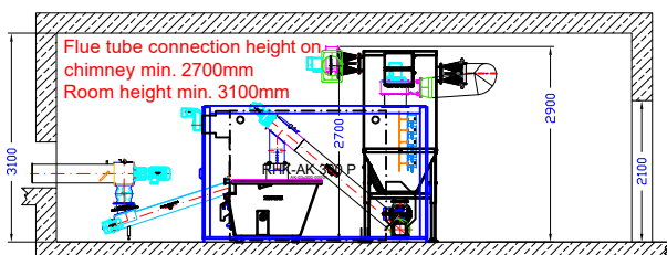
Multicyclone with de-ashing 900 Liter
