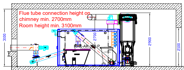
Multicyclone with separate de-ashing 240 Liter Boiler ash bin 900 Liter
