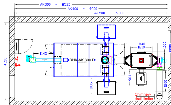
Multicyclone with separate de-ashing 240 Liter Boiler ash bin 900 Liter
